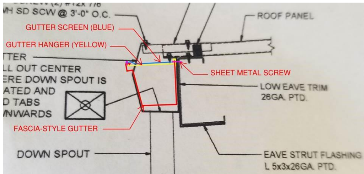
Figure 1. Schematic Mt. Gilead Water Conservation Project pavilion gutter detail
